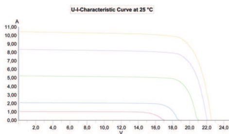
U-I-Characteristic Curve 100 W/m 2 , U-I-Characteristic Curve 200 W/m 2 , U-I-Characteristic Curve 500 W/m 2 , U-I-Characteristic Curve 800 W/m 2 , U-I-Characteristic Curve 1 000 W/m 2
